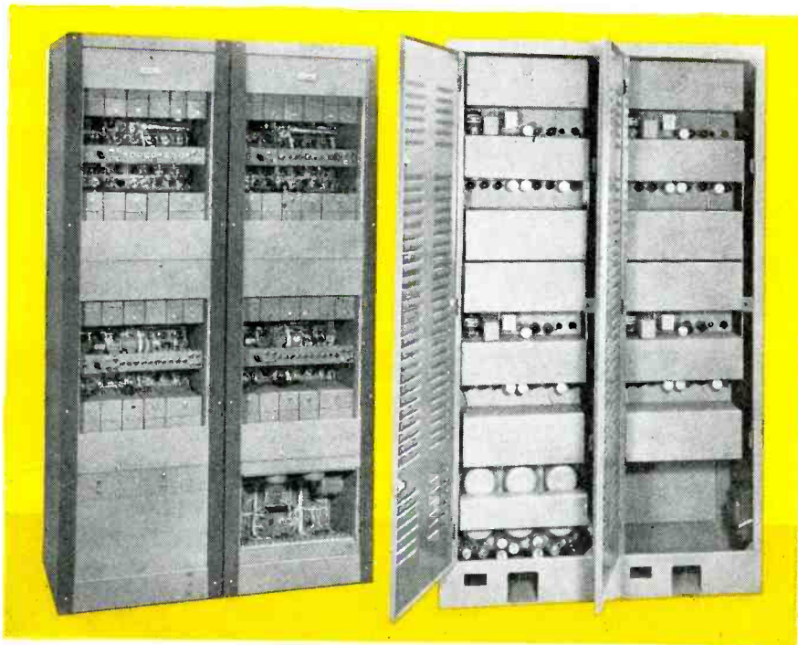
Front view with covers removed, and rear view of the four terminal carrier equipment which provides four complete communication channels and termination to two-wire line
