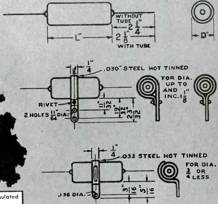
Class 23M—One terminal grounded (with insulating tube)
