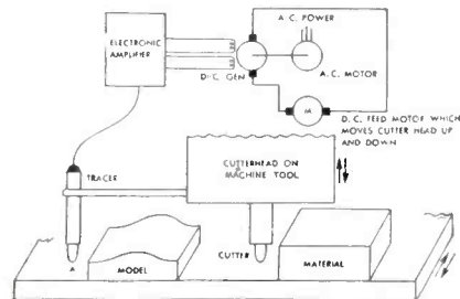
Tube-controlled tracer mechanism for intricate surface-machining
