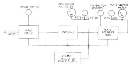
Fig. 3. Block diagram of the vacuum tube voltmeter designed to measure very low frequencies
