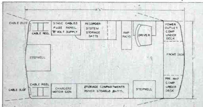
Plan of vehicle showing arrangement of batteries, power equipment and cable reels, etc. At right, the battery compartment from the inside with the soundproof motor-generator compartment adjacent
