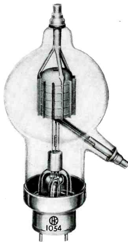
Fig. 3—HK-1054, 750-watt tantalum tube
