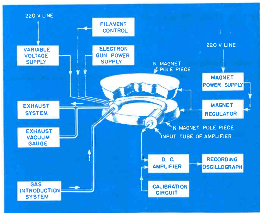
A Fig. 3—Block diagram of mass spectrometer equipment showing tube between poles of magnet
