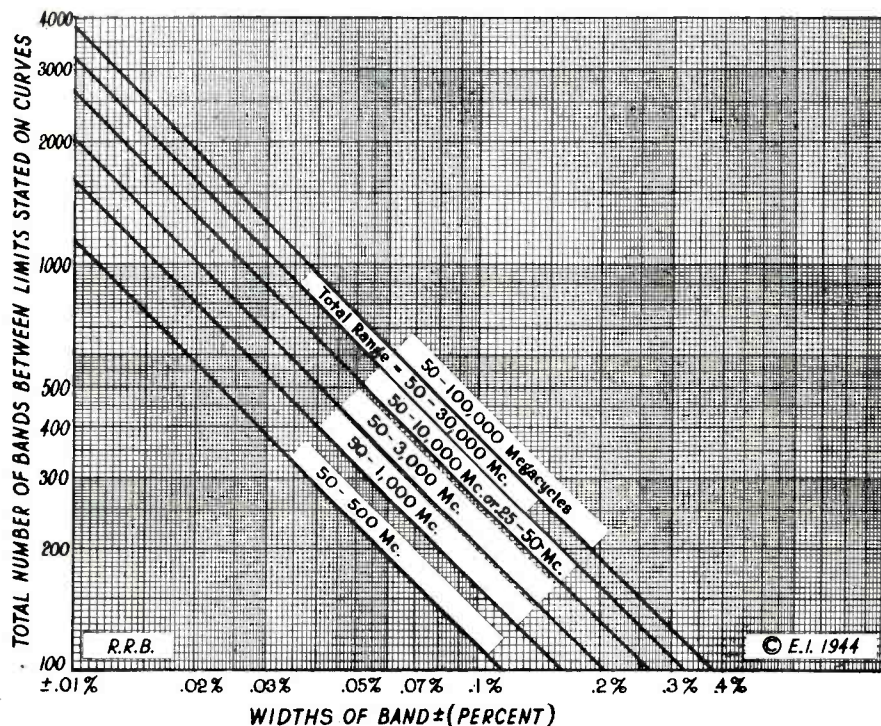
Showing number of useful communication channels which become available when the width of the band is limited to various percentages of the fundamental frequency
