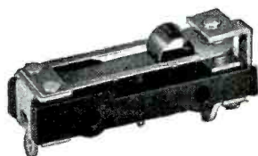
Acro Midget Switch Designed With Actuating Pin Below. 10 Amps at 115 Volts A. C. 1½" long.
