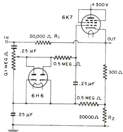
Expansion unit diagram
