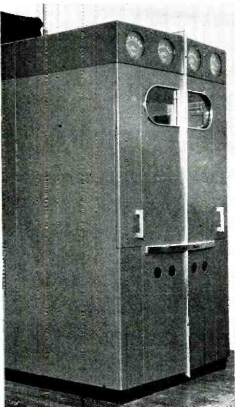
The model 503A Western Electric FM transmitter feeds antenna through coaxial line
