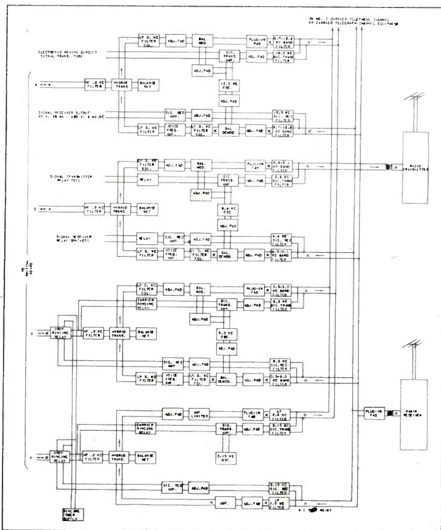
Block diagram of four (or more) two-way carrier channels applied to radio system
