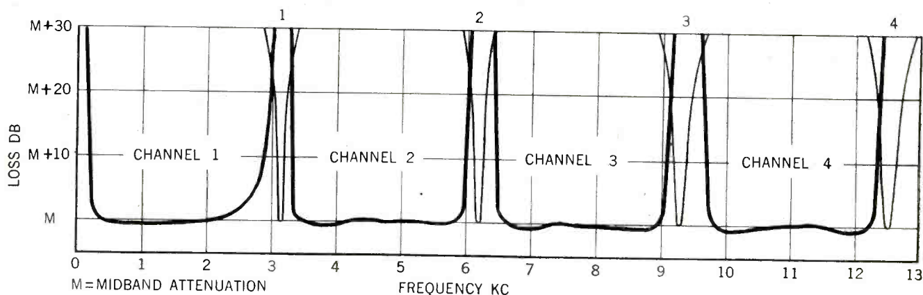
Relative overall transmission frequency characteristics of four-channel radio carrier telephone system. Channel bandwidths are representative of overall audio transmission characteristics measured between two-wire terminations
