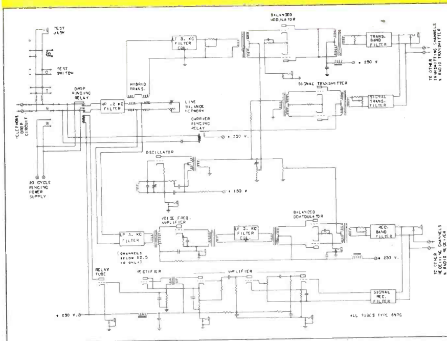
Basic circuit diagram for one channel of system shown in block diagram above
