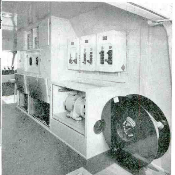
Plan of vehicle showing arrangement of batteries, power equipment and cable reels, etc. At right, the battery compartment from the inside with the soundproof motor-generator compartment adjacent
