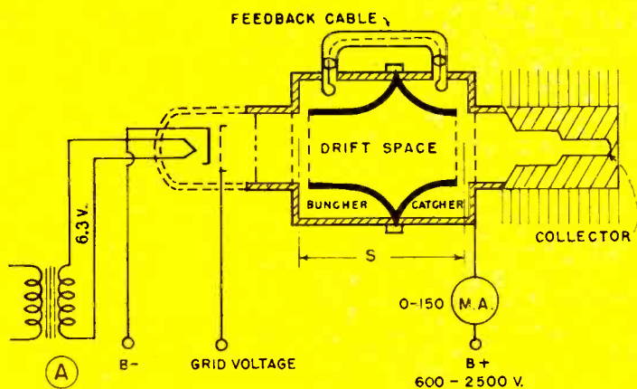
Fig. 7. Klystron tube at A showing bunching distance S and equivalent conventional tube circuit at B. Phase-shift network replaces drift space
