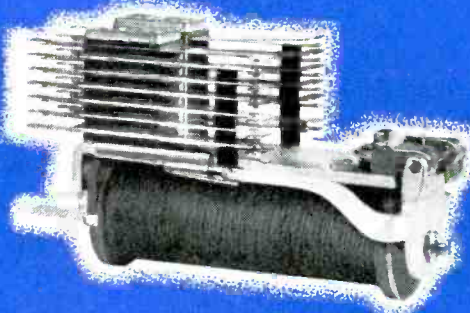
ABOVE—Type 142—Double pile-up relay on large telephone type frame, representing approximately the maximum number of spring combinations.
