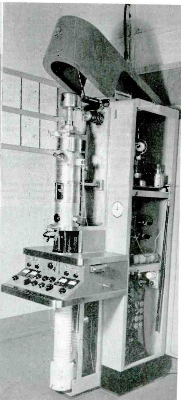
Type EMU is the universal RCA model, shown open, and has been considerably revised to simplify getting it into operation
