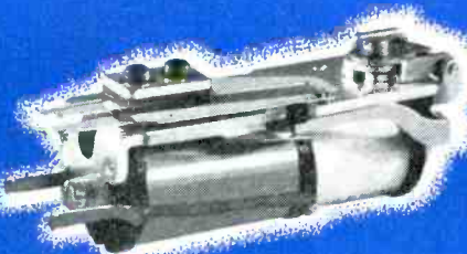
ABOVE—Type 132—Time delay relay of the slug type. Pure copper slug on heel end of core provides maximum of 300 milli-seconds delay in contact opening after circuit is broken.
