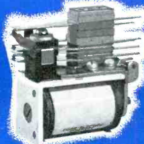
ABOVE—Type 108—Antenna switching contact combination with Mycalex insulation. Has a side contact mount to reduce capacity between antenna circuit and ground.
