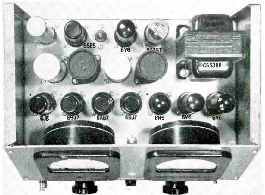
Looking down on the chassis showing the tube arrangement of the instrument which is described as a plate rectifier slide-back vacuum tube voltmeter
