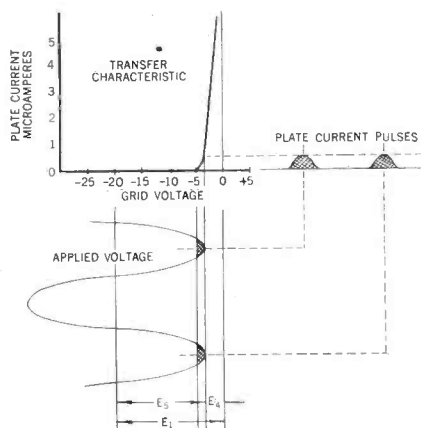
Fig. 2—Graphic presentation of operation. Transfer characteristic of the tube for the applied plate potential is plotted
