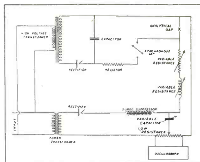
Basic circuit of the multisource spectrographic excitation unit
