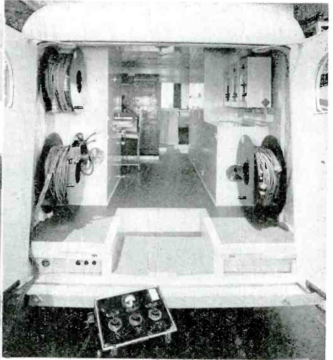
Interior view of the mobile studio showing stepwell, cable reels and general arrangement of the complete equipment
