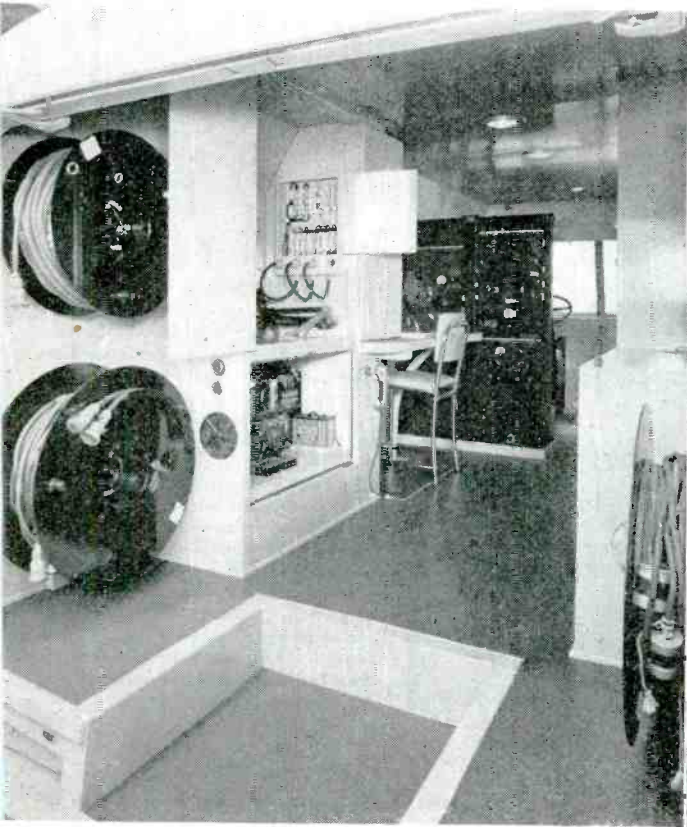
Cable reels, provided with brakes, are at the left rear with motor generator and B battery compartment just ahead
