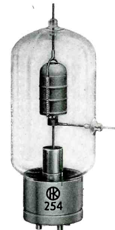
Fig. 2—HK-254, 100-watt tantalum tube
