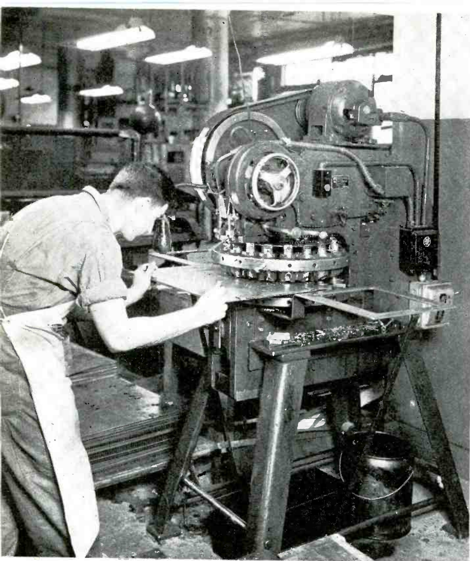
PUNCHING 100 HOLES in radio chassis needed in small lots at Federal Telephone and Radio Corp., Newark, N. J., with turret-head punch press designed for short run piercing operations
