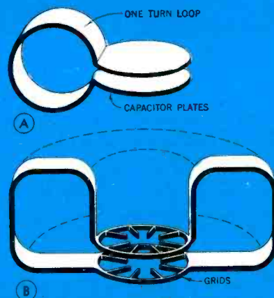
Fig. 4—Simple tank circuit at A has low Q at uhf because of radiation of energy. Increasing number of loops as at B develops into cavity as used in Klystron and other tubes
