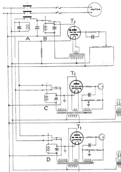
Schematic of revolving door control system
