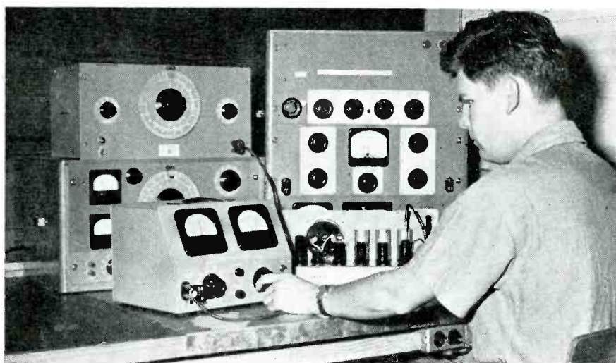
General view of the low frequency voltmeter (instrument with sloping panel) in use for the measurement of the low frequency characteristics of an amplifier
