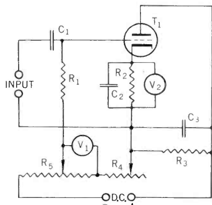
Fig. 1—Schematic showing the components in the vacuum tube voltmeter for low frequencies
