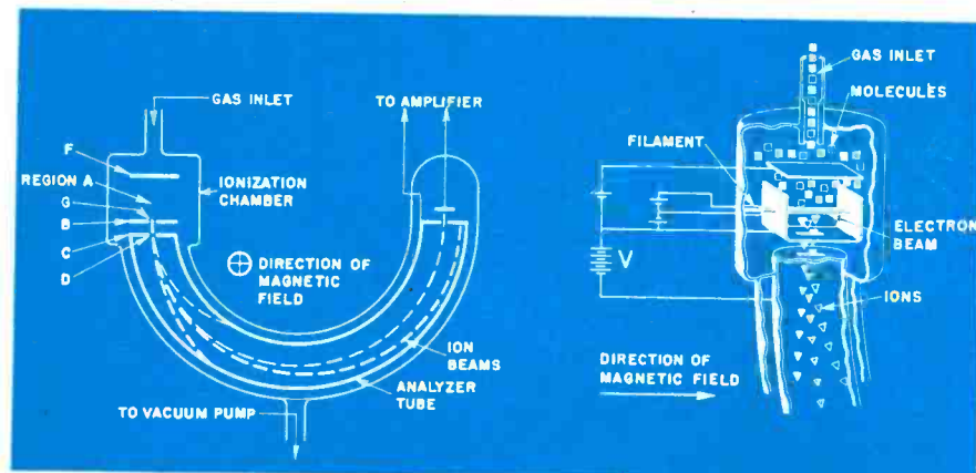
Fig. 2—Details of region A in Fig. 1. Electron beam ionizes gas sample by collision. Voltage V gives forward velocity to ions which in combination with magnetic field and their mass determine path radius
