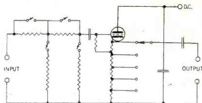
Fig. 4. Input circuit of the low frequency VTVM, which uses a ladder type divider
