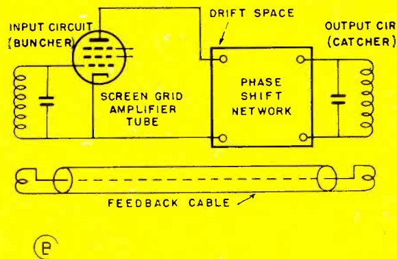
Fig. 7. Klystron tube at A showing bunching distance S and equivalent conventional tube circuit at B. Phase-shift network replaces drift space
