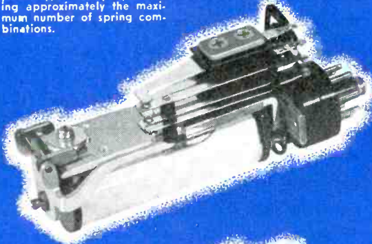
ABOVE—Type 113—An A.C. relay having a laminated core, heavy Oilite bearing yoke, special silicon steel armature and heel piece, and plug-in base.
