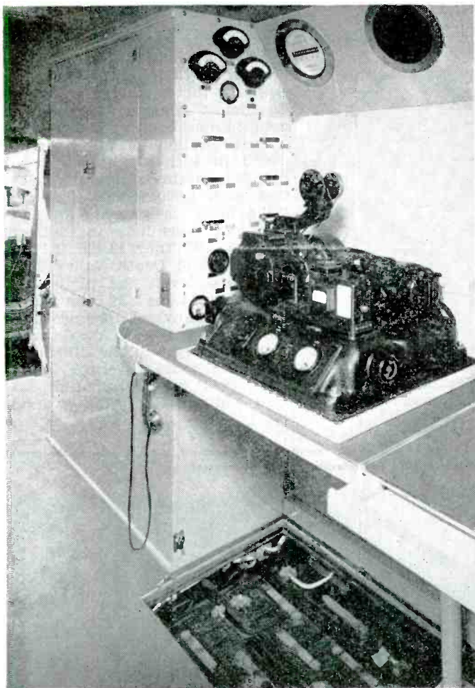
The sound film track recording equipment is mounted on a convenient shelf with its controls and meters built into the bulkheads adjacent to it. Beneath the machine one of the below-floor externally accessible battery compartments is shown with the floor up
